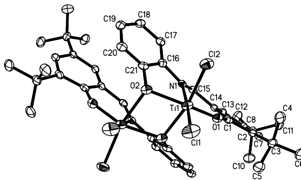
Fig. 3. An ORTEP diagram of the molecular structure of 4 showing 50% thermal ellipsoid probabilities.
