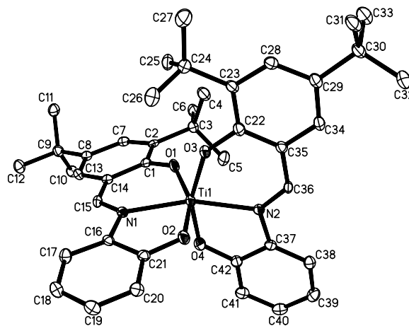
Fig. 4. An ORTEP diagram of the molecular structure of 6 showing 50% thermal ellipsoid probabilities.
