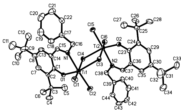
Fig. 2. An ORTEP diagram of the molecular structure of 3 showing 50% thermal ellipsoid probabilities.
