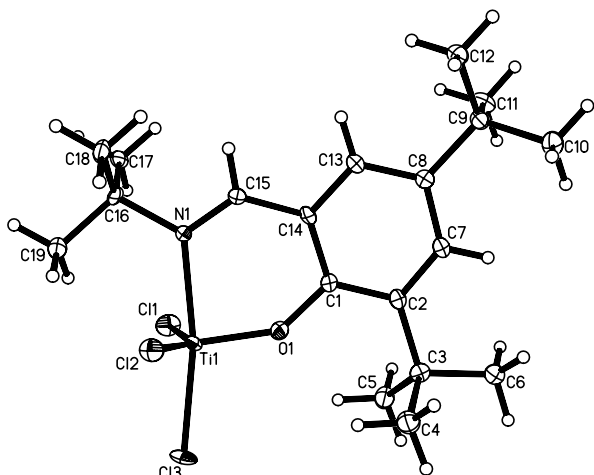
Fig. 1. An ORTEP diagram of the molecular structure of 2 showing 50% thermal ellipsoid probabilities.
