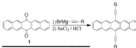
Scheme 1. Functionalized Pentacene Synthesis
