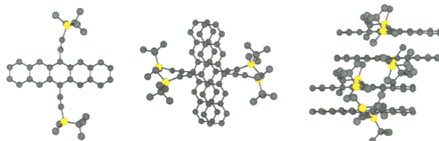
Figure 5. Crystallographic order of compound 6' (second polymorph of 6 ). Left: Single molecule showing distorted alkynes. Middle: View down a column of pentacene units. Right: Columnar order, view down the pentacene short axis.
