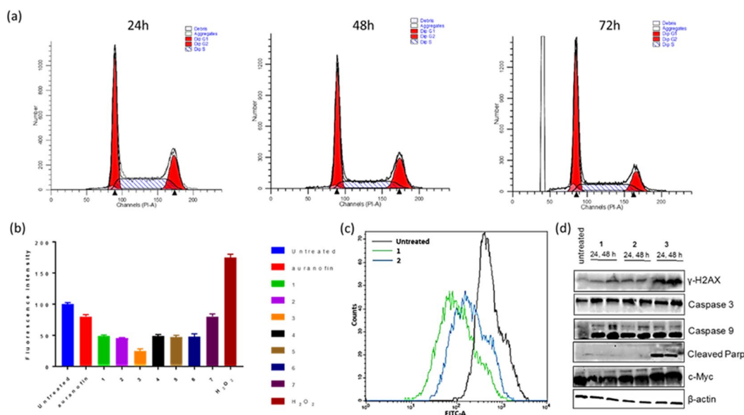
Figure 10. (a) Histogram representing the different phases of the cell cycle of OVCAR8 in the presence or absence 1 (2 \mu M) over the course of 72 h. 24 h treated with 1 : G1: 42.22%, S: 36.39%, G2/M: 21.38%, 48 h treated with 1 : G1: 47.27%, S: 34.46%, G2/M: 18.26%, 72 h treated with 1 : G1: 54.99%, S: 29.48%, G2/M: 15.53%. (b) Intracellular ROS using OVCAR8 cells and dihydrorhodamine 123 as dye. Plots show untreated cells (negative control), H 2 O 2 treated cells (positive control), and cells treated with 1 – 7 (5 \mu M, overnight) or auranofin (5 \mu M, overnight). (c) Histogram plot of the effects of 1 and 2 ( \mu M) on mitochondrial membrane potential using rhodamine 123 in OVCAR8 cells. (d) immunoblotting for the expression of apoptosis and DNA damage response proteins in OVCAR8 cells following incubation with 1 , 2 , or 3 . (full-length blots/gels are presented in Supplementary Fig. 68).
