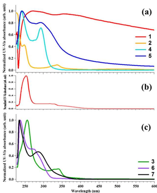
Figure 2. UV-Vis absorption spectrum of Au(I) series, 1 , 2 , 4 , and 5 in PBS ( a ), 1 in CHCl 3 ( b ), Au(III) series, 3 , 6 , and 7 in PBS ( c ). Concentration of complexes = 50 \mu M. DMSO was used for stock solution. (The final concentration of DMSO was 1% of the total solution).
