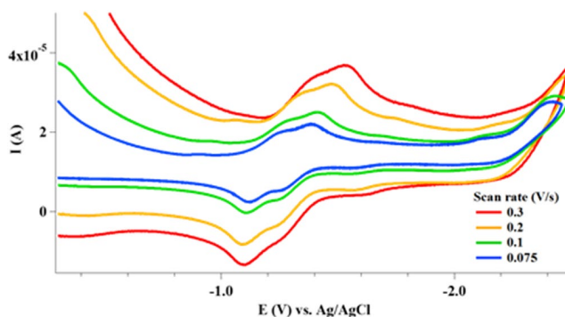
Figure 6. Cyclic voltammograms recorded at a platinum electrode in DMSO solution of 1.0 mM 2 , with \text{NaClO}_4 supporting electrolyte; scan rate 0.3, 0.2, 0.1, and 0.075 \text{V sec}^{-1} .
