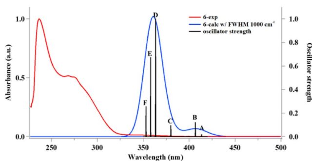
Figure 3. UV-Vis absorption spectrum of Au(III) complex, 6 , in PBS at the concentration of 50 \mu M. DMSO was used for stock solution (red) and theoretical spectrum (blue) and oscillator strengths, f , from Table 1 for 6 (black).
