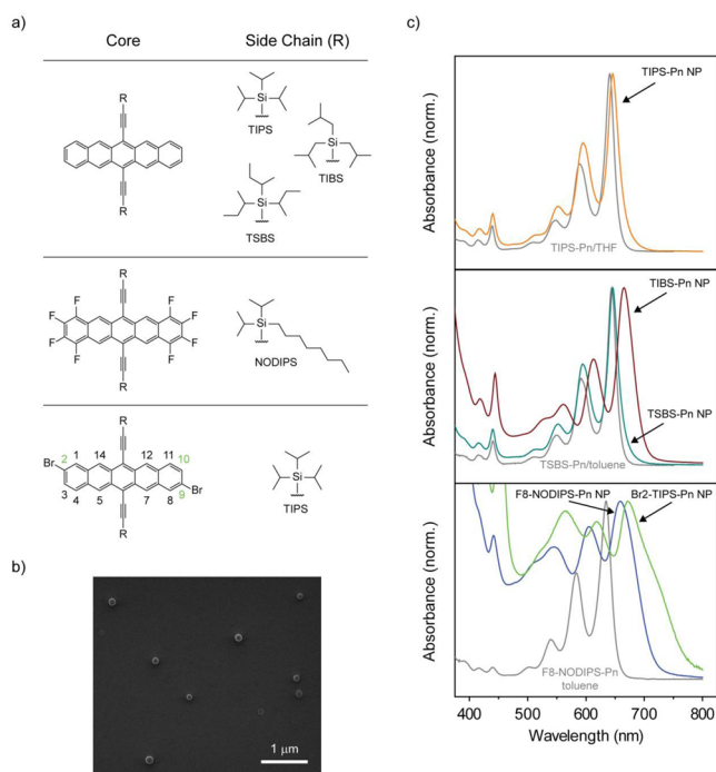
Figure 1. Pentacene derivatives and their nanoparticles. (a) Core structure and side chains (including acronyms) of the pentacene derivatives. (b) SEM image of ~100 nm diameter TIBS-pentacene nanoparticles. (c) Steady-state absorption spectra of TIPS-pentacene in THF and aqueous colloidal TIPS-pentacene nanoparticles (top panel), TSBS-pentacene in toluene and aqueous colloidal TSBS- and TIBS-pentacene nanoparticles (middle), and F8-NODIPS-pentacene in toluene and aqueous colloidal F8-NODIPS- and Br2-TIPS-pentacene nanoparticles (bottom panel). The absorption spectra of TIBS- and Br2-TIPS-pentacene in toluene have been omitted for clarity. The TIPS- and TSBS-pentacene nanoparticle absorption spectra exhibit a slight redshift relative to the absorption spectrum of the corresponding pentacene derivative dissolved in either THF or toluene. The TIBS-, F8-NODIPS-, and Br2-TIPS-pentacene nanoparticle absorption spectra are more substantially red-shifted and exhibit broader spectral features. Splitting of the 0–0 band in the Br2-TIPS-pentacene nanoparticle absorption spectrum is apparent.
