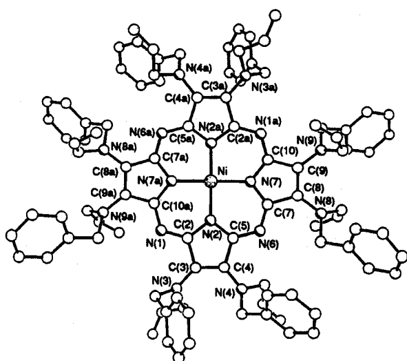
Fig. 2 X-ray crystal structure of {2,3,7,8,12,13,17,18-octakis[allyl(benzyl)amino]porphyrinato}nickel(II)
