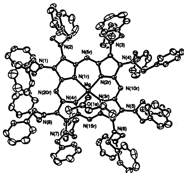
Fig. 1 X-ray crystal structure of [2,3,7,8,12,13,17,18-octakis(dibenzylamino)porphyrinato]magnesium(II)
