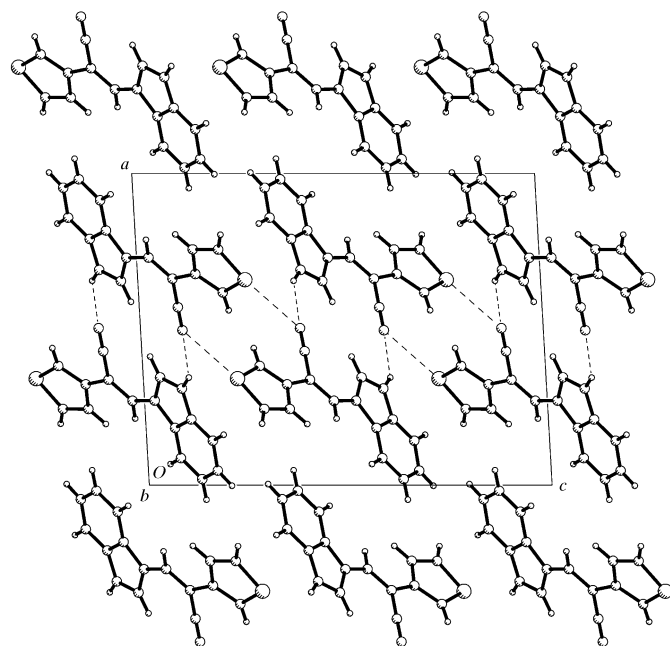
Figure 3 A packing diagram of (I), viewed down the b axis, showing hydrogen-bonding interactions (dashed lines).
