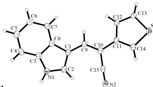
Figure 1 A view of the molecule of (I), showing the atom-numbering scheme. Displacement ellipsoids are drawn at the 50% probability level and H atoms are shown as small spheres of arbitrary radii. The thienyl ring is disordered and only the ring with the major occupancy [0.944 (2)] is shown.
