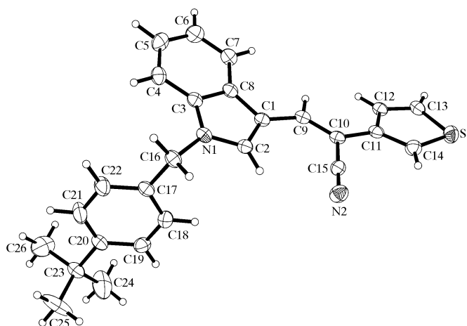
Figure 2 A view of the molecule of (II), showing the atom-numbering scheme. Displacement ellipsoids are drawn at the 50% probability level and H atoms are shown as small spheres of arbitrary radii. The methyl groups of the tert -butyl moiety are disordered over two orientations and only the groups with the major occupancy [0.668 (6)] are shown.
