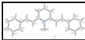
Fig. 1. A view of the molecule with the atom numbering scheme. Displacement ellipsoids are drawn at the 50% probability level.
